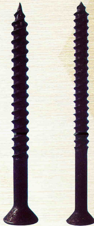
© Various Flat Head & Bugle Head TWINFAST TWIN LEAD SMS, 2/3 THREAD LENGTH.
